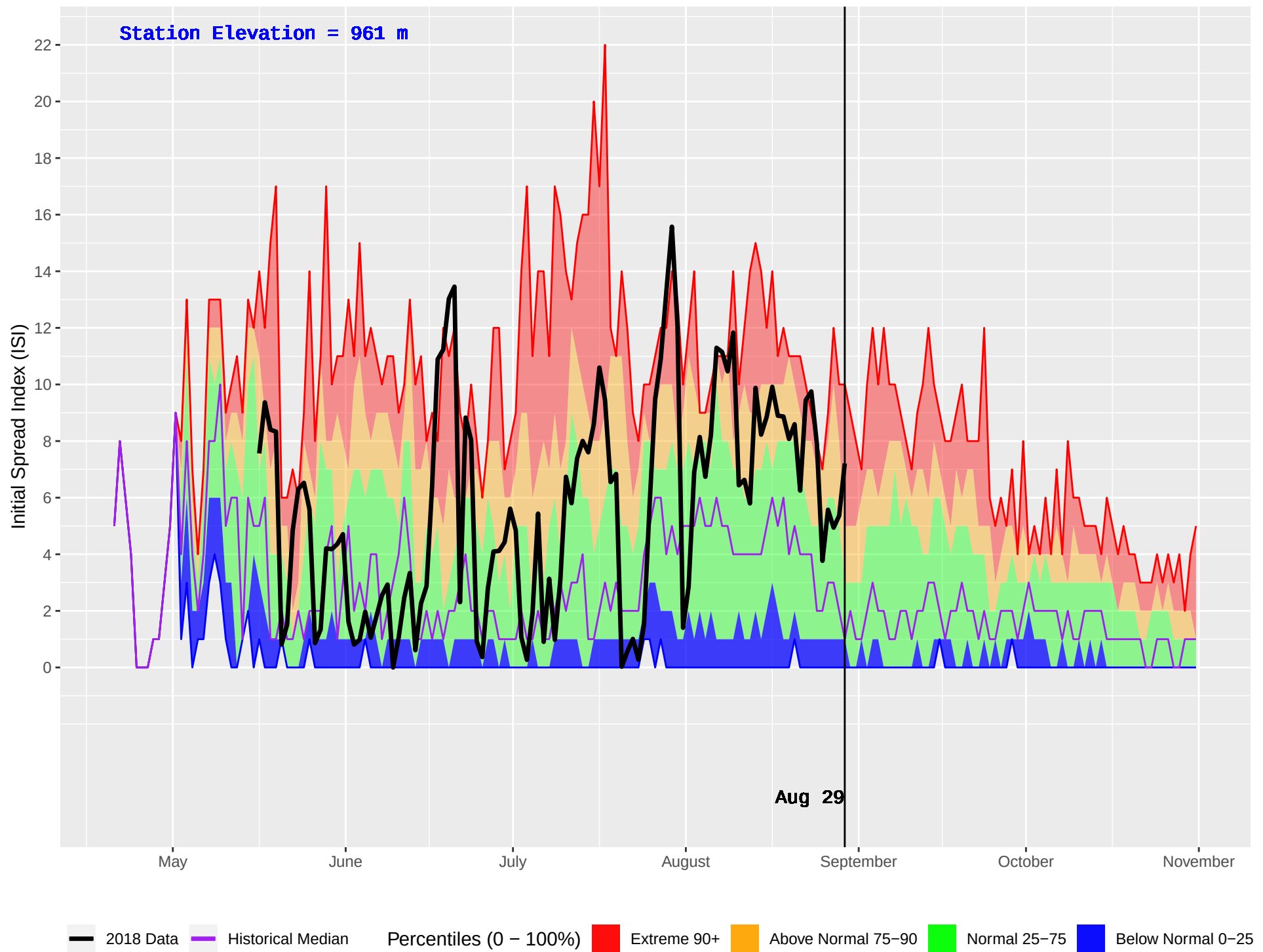
HOLY CROSS 2 (654) : Historical (1998–2016) and Current (2018) Daily Initial Spread Index (ISI)
