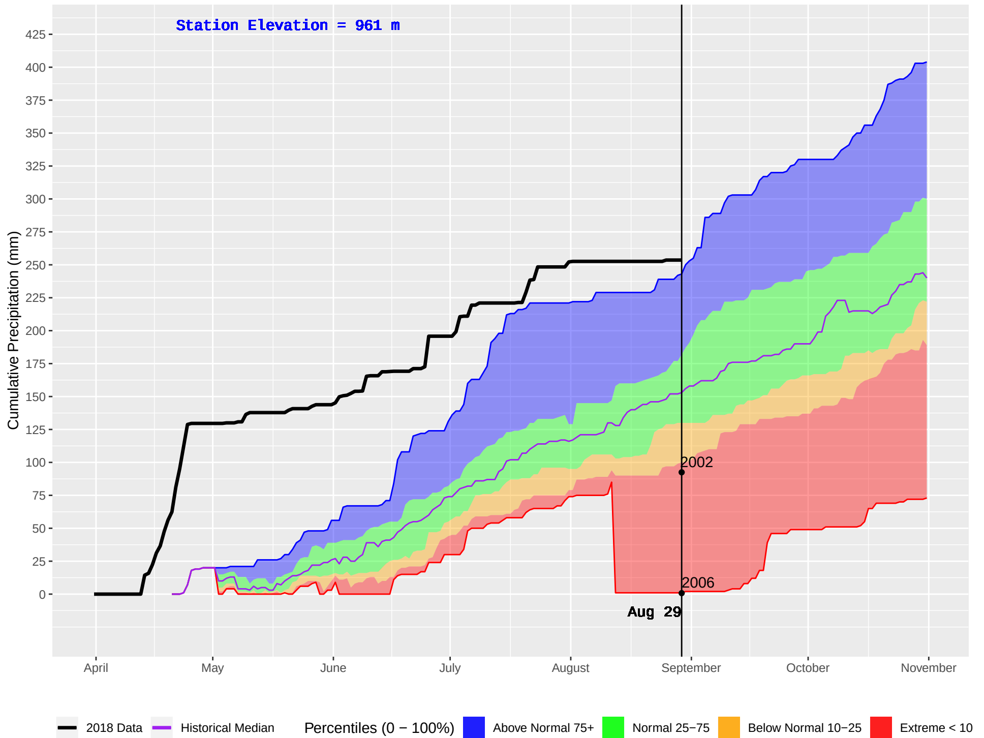
HOLY CROSS 2 (654) : Historical (1998–2016) and Current (2018) Daily Cumulative Precipitation
