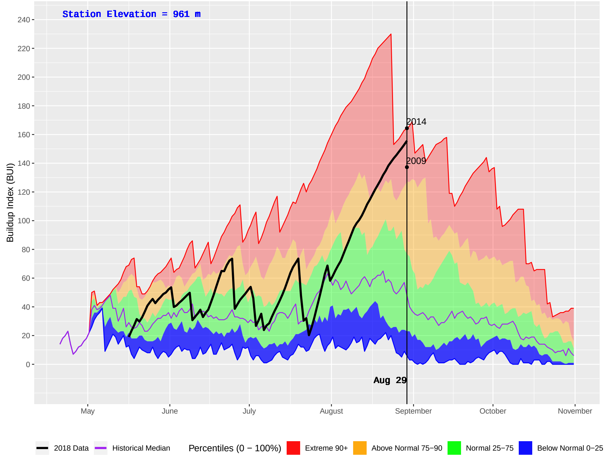
HOLY CROSS 2 (654) : Historical (1998–2016) and Current (2018) Daily Buildup Index (BUI)
