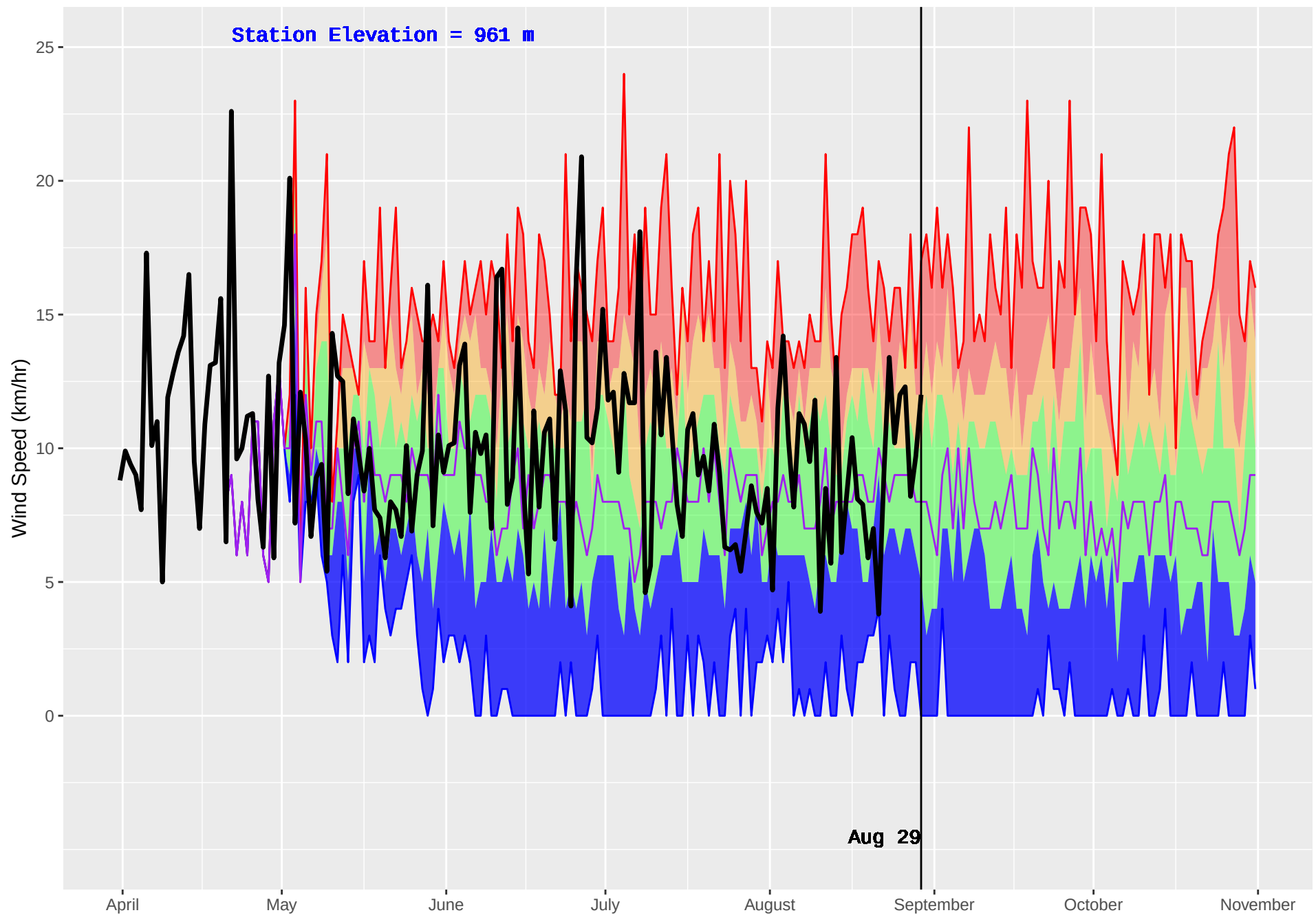
HOLY CROSS 2 (654) : Historical (1998–2016) and Current (2018) Daily Wind Speed
