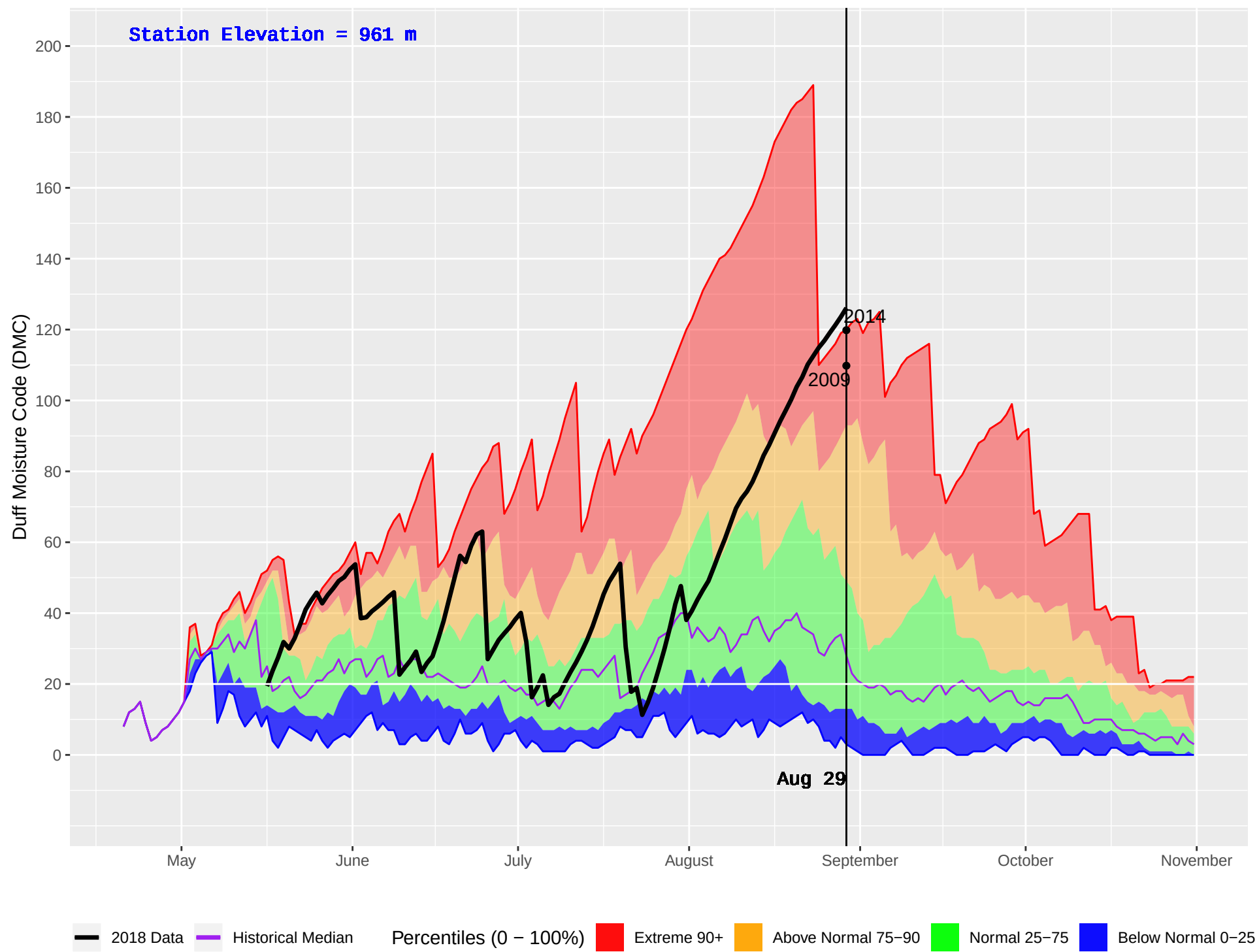
HOLY CROSS 2 (654) : Historical (1998–2016) and Current (2018) Daily Duff Moisture Code (DMC)
