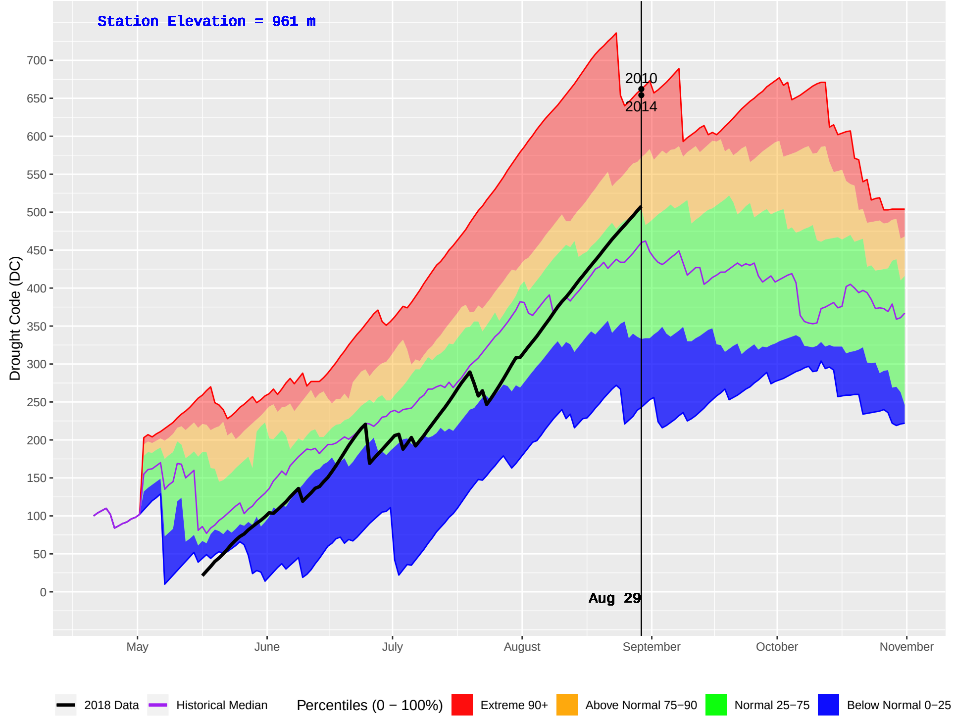
HOLY CROSS 2 (654) : Historical (1998–2016) and Current (2018) Daily Drought Code (DC)
