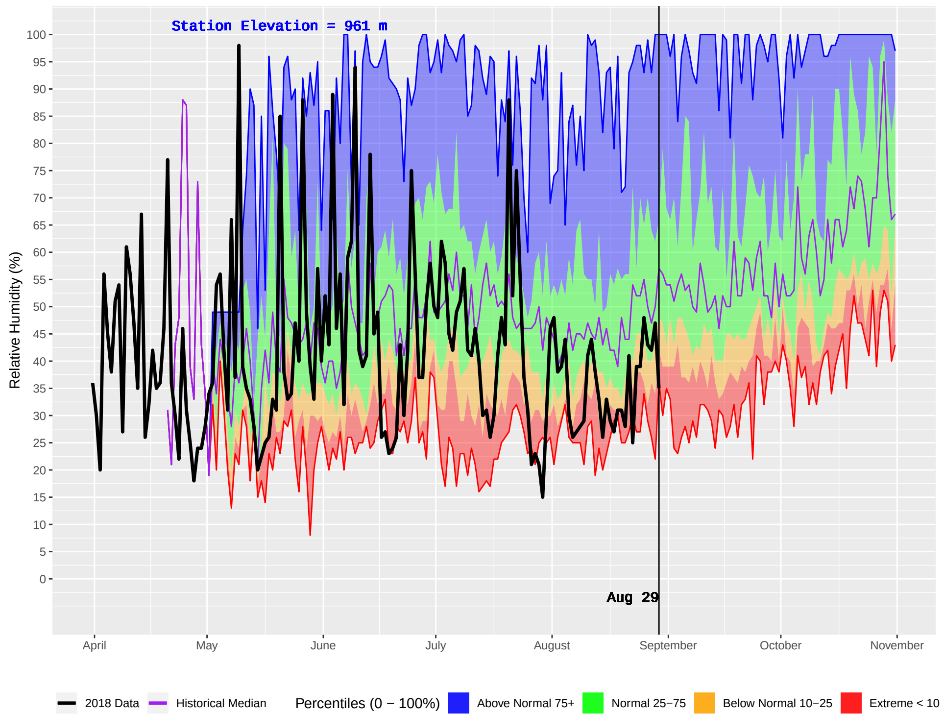
HOLY CROSS 2 (654) : Historical (1998–2016) and Current (2018) Daily Relative Humidity
