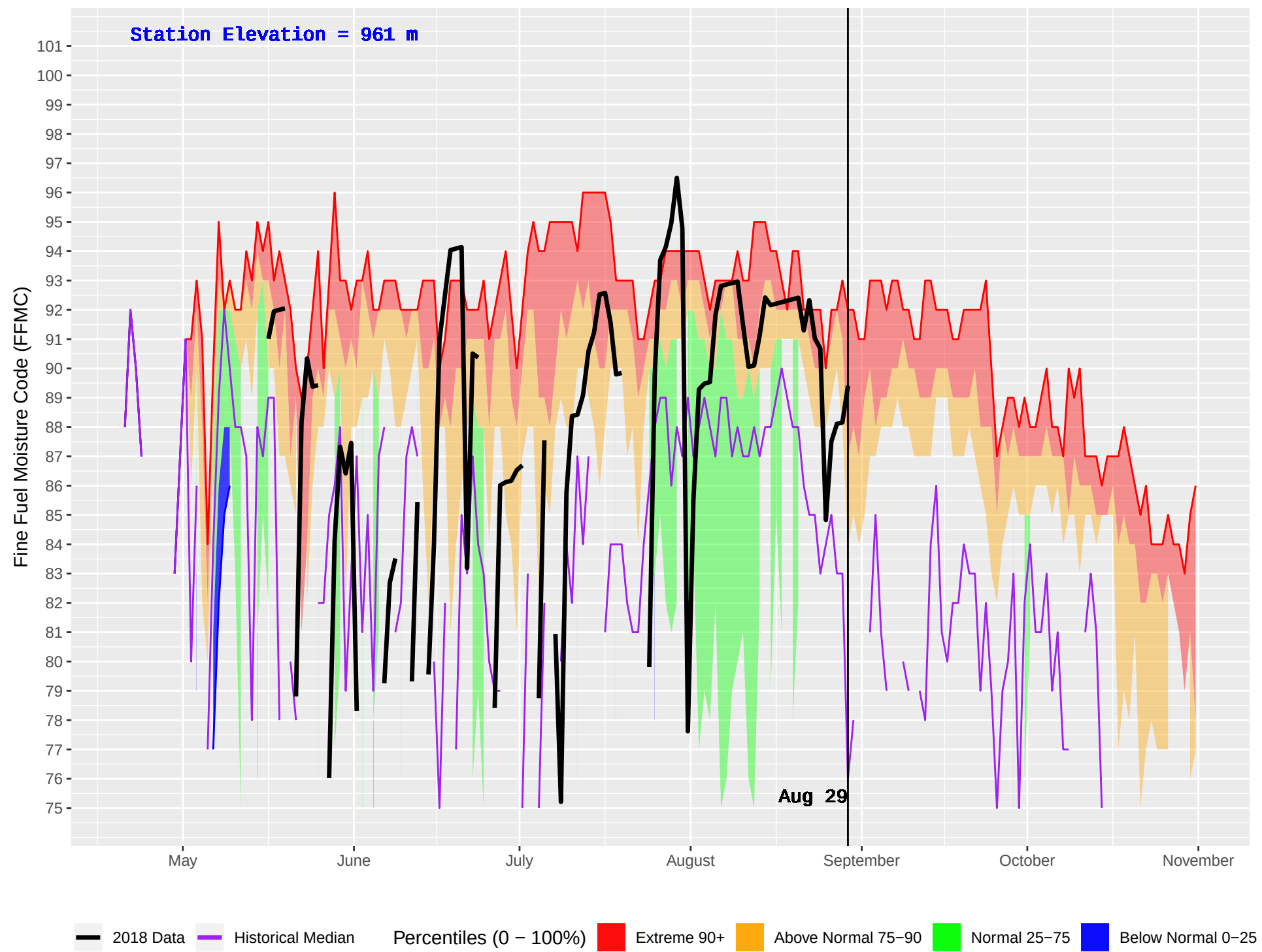
HOLY CROSS 2 (654) : Historical (1998–2016) and Current (2018) Daily Fine Fuel Moisture Code (FFMC)
